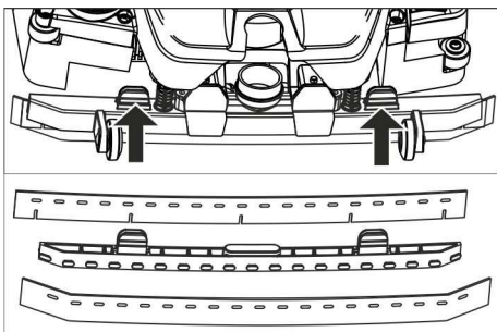
1 Skruv 2 Lock
